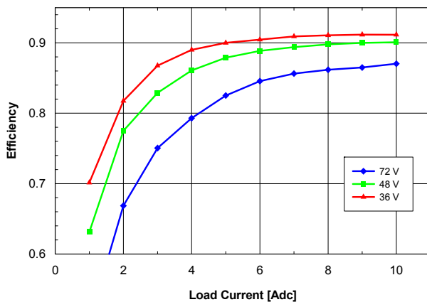
Figure 2. Efficiency vs. load current and input voltage for SSQE48T10033 converter mounted vertically with air flowing from pin 1 to pin 3 at a rate of 300 LFM (1.5 m/s) and Ta=25°C.
