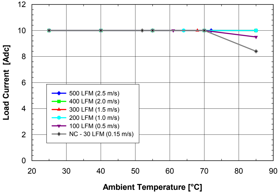
Figure 1. Available load current vs. ambient air temperature and airflow rates for SSQE48T10033 converter mounted vertically with air flowing from pin 1 to pin 3, Vin = 48 V. Note: NC – Natural convection
