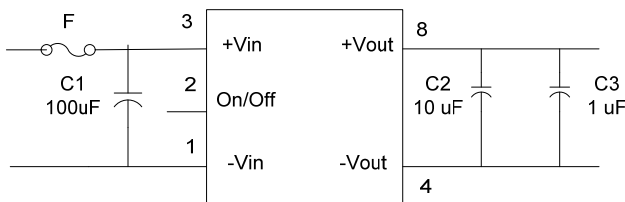
Figure 2. Typical Application of QTS48T25120
