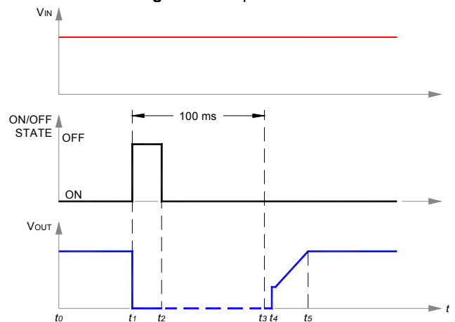
Fig. G: Start-up scenario #
