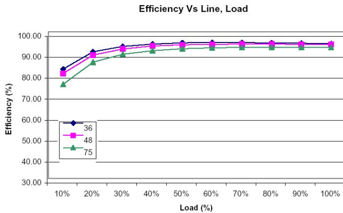
Figure 1. QKS48T21120 Efficiency vs. Output Load
