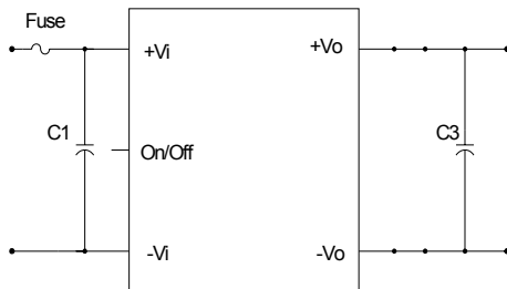
Figure 2. Typical Application of QKS48T21120
