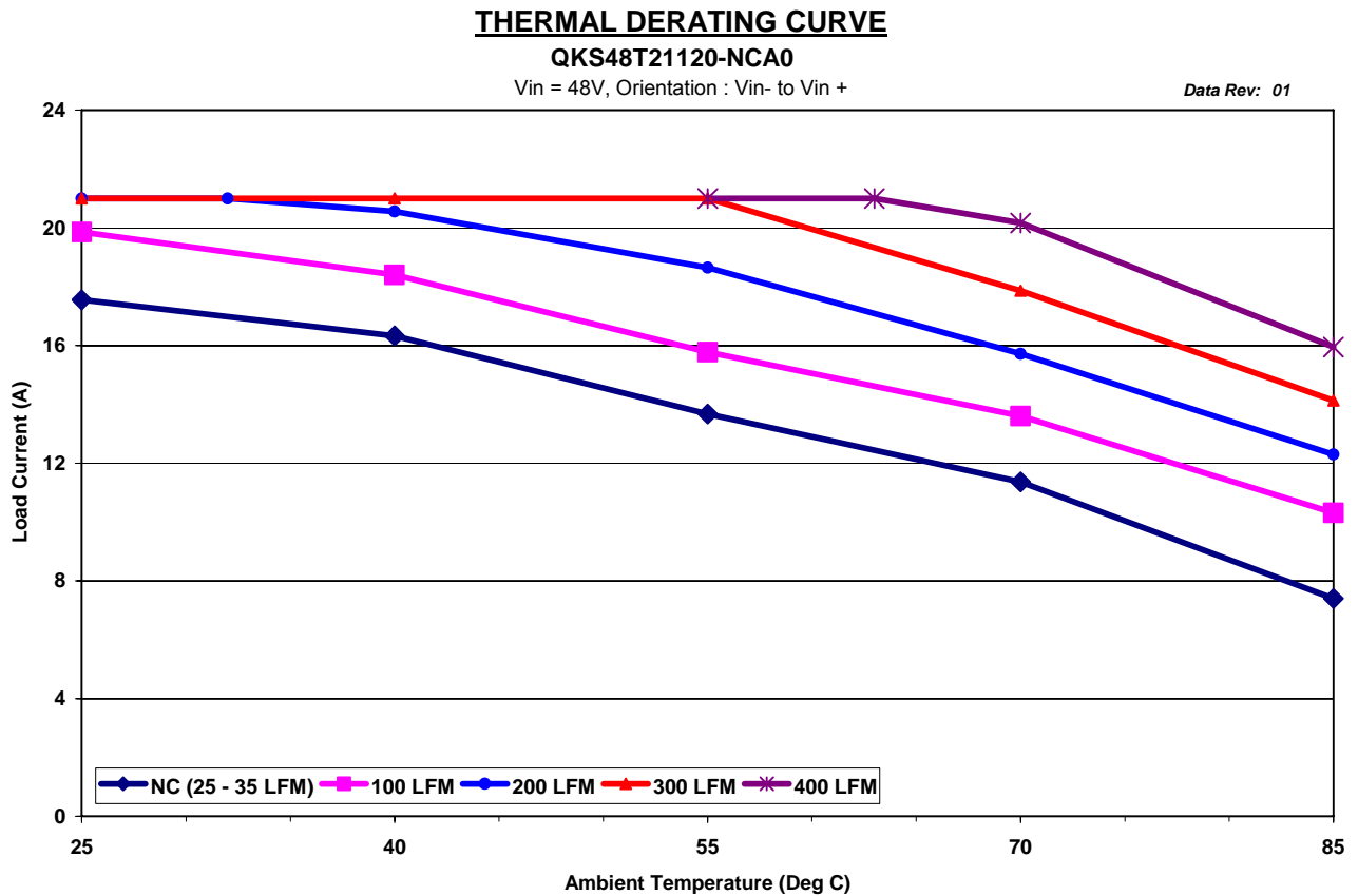
Figure 3. QKS48T21120 Derating Curves
