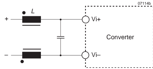
Fig. 15 External circuitry to comply with EN 55011/55022, level B, radiated
