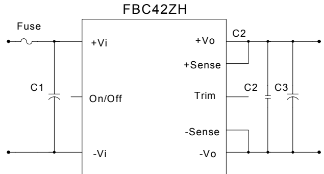
Figure 3. Typical Application of FBC Series
