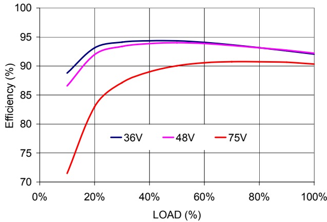
Figure 1. FBC42ZH Efficiency Vs. Output Load
