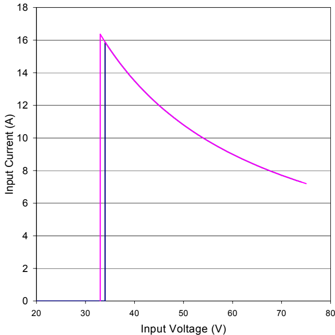
Figure 2. FBC42ZH Input Characteristic
