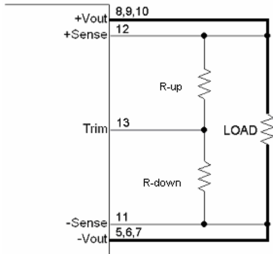
Figure 4. FBC Series Positive Trim Schematic
