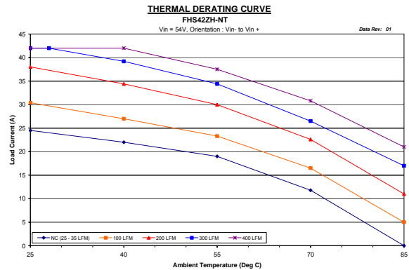
Figure 5. FBC42ZH Derating Curves
