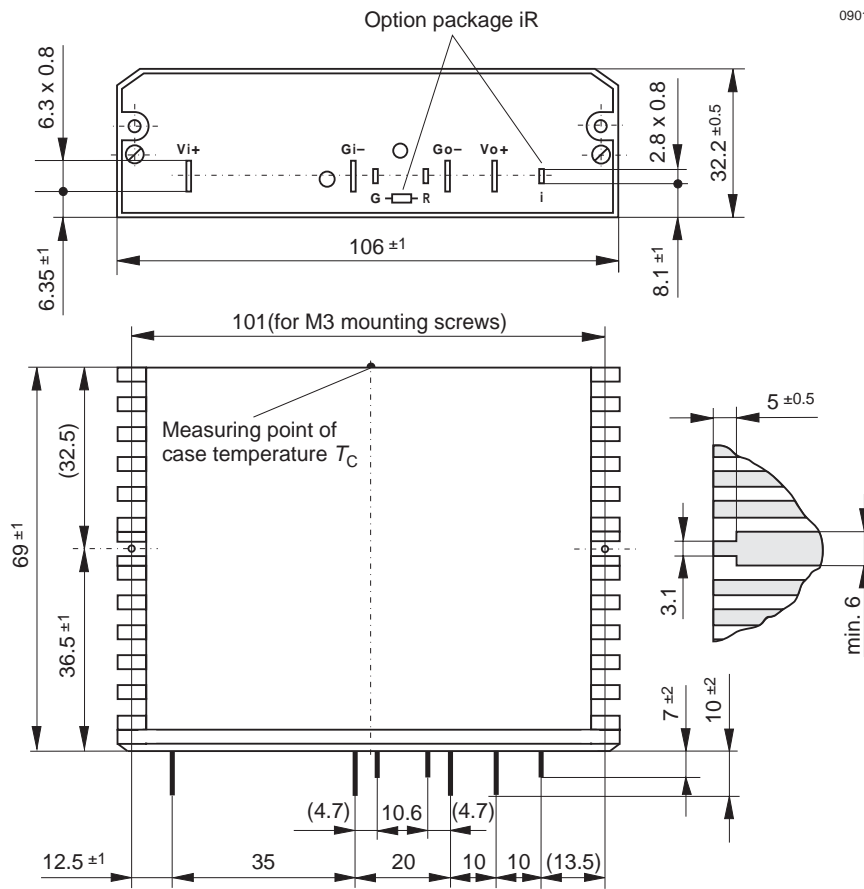
Fig. 6 Case B02, weight 230 g Aluminium, black finish and self cooling
