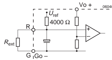
Fig. 8 Voltage adjustment with external resistor R_{\text{ext}}
