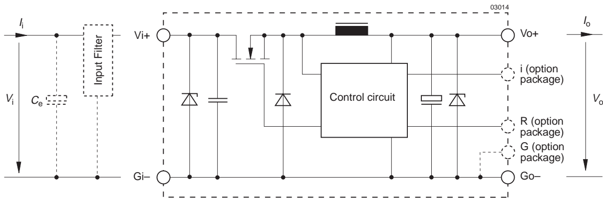
Fig. 1 Block diagram
