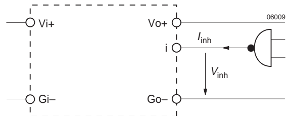
Fig. 10 Definition of I_{\text{inh}} and V_{\text{inh}}
